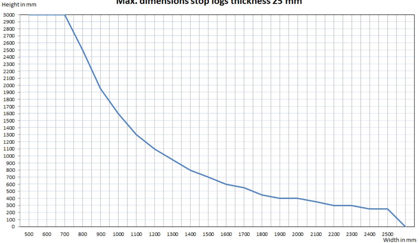
Max. dimensions stop logs thickness 25 mm
