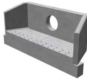
N27A 1300mm Backwall
